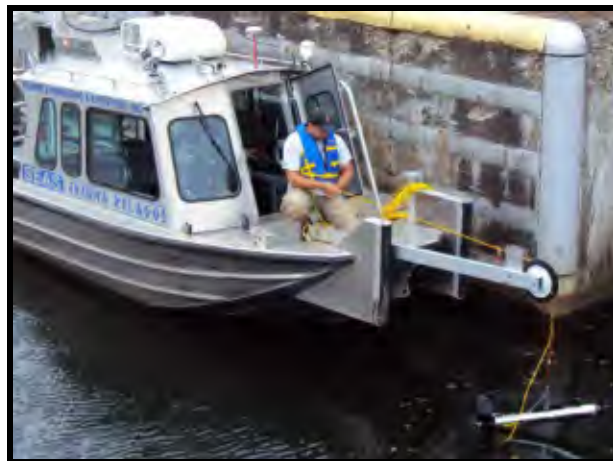
EdgeTech Towfish mounted off the bow
